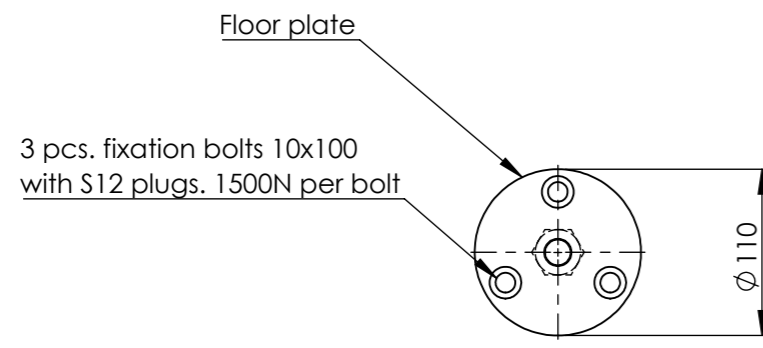
Topview of floorplate
